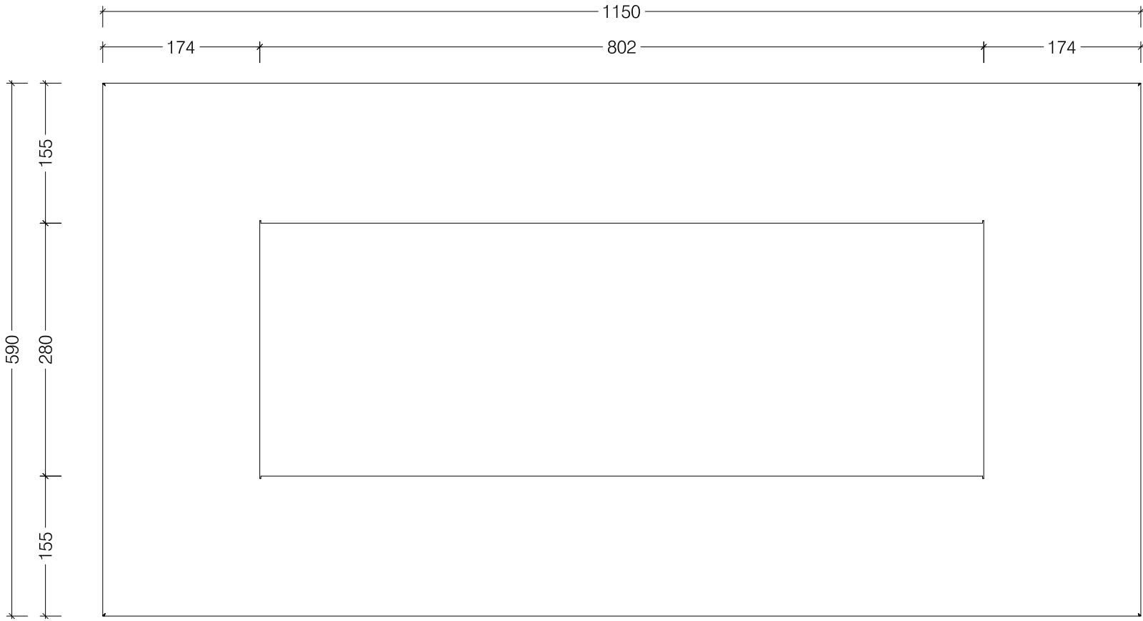
Front View
