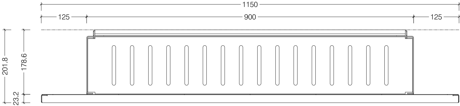
Top View
